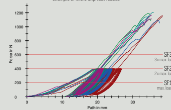
example of Micro Grip test results
